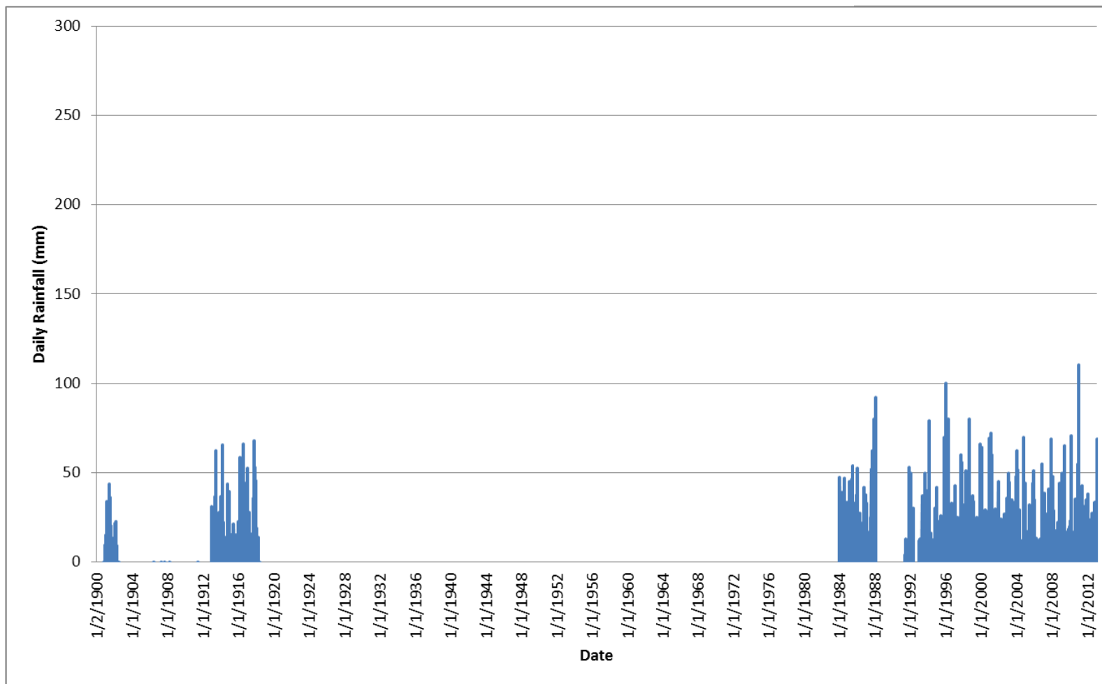
FIGURE B-8 DAILY RAINFALL: CECIL PLAINS HOMESTEAD (41016), 1900-2012
