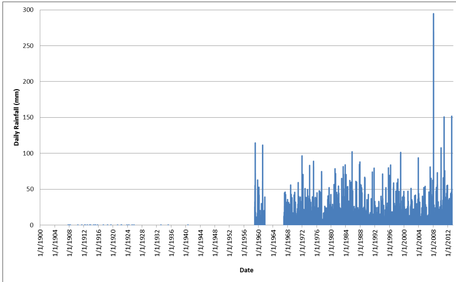
FIGURE B-20 DAILY RAINFALL: DAANDINE (41297), 1900-2012
