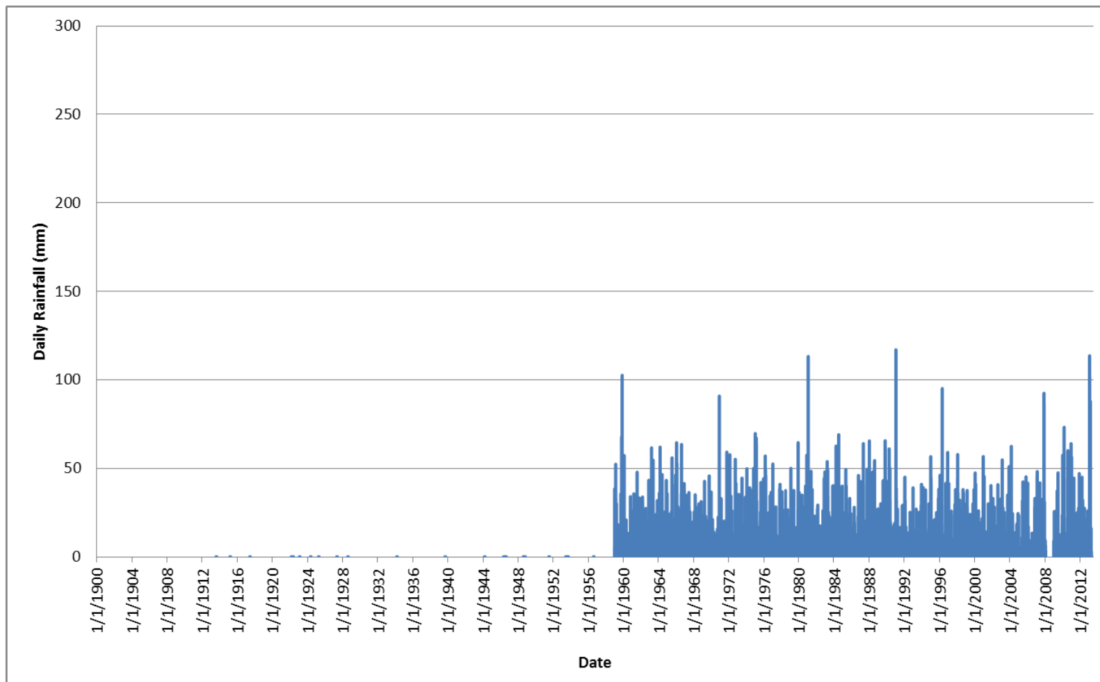
FIGURE B-19 DAILY RAINFALL: ROSEVALE (41168), 1900-2012
