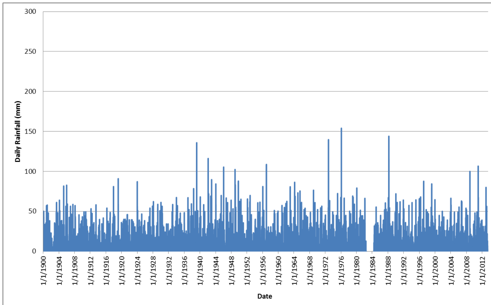
FIGURE B-17 DAILY RAINFALL: PRATTEN (41083), 1900-2012
