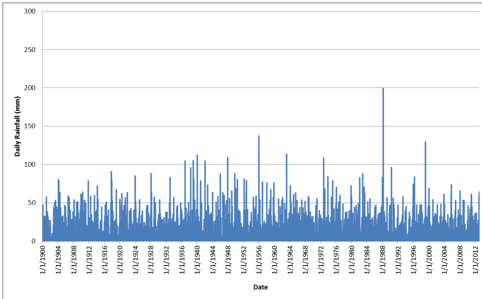
FIGURE B-15 DAILY RAINFALL: LEYBURN POST OFFICE (41063), 1900-2012
