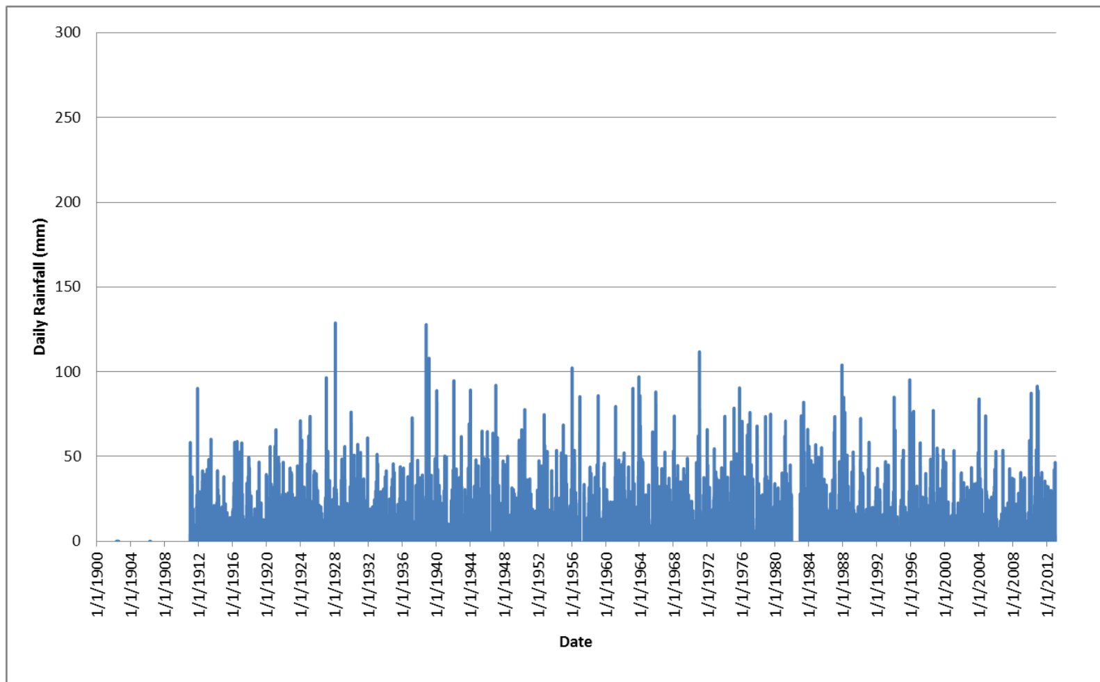
FIGURE B-10 DAILY RAINFALL: CONDAMINE PLAINS (41019), 1900-2012
