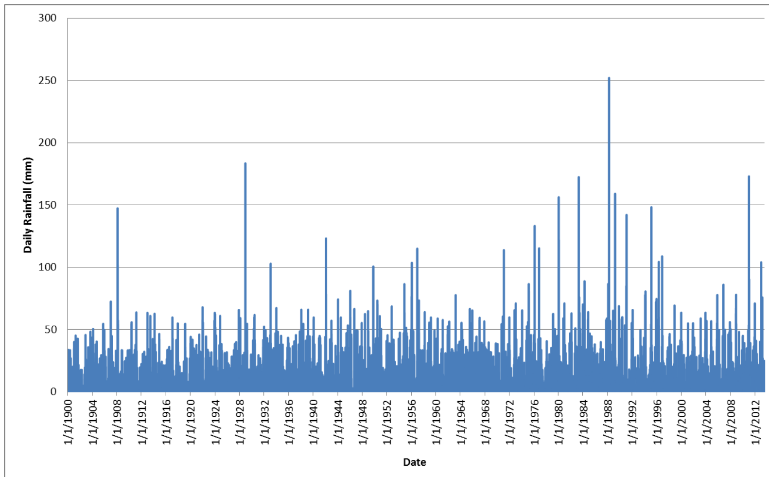
FIGURE B-9 DAILY RAINFALL: CLIFTON POST OFFICE (41018), 1900-2012
