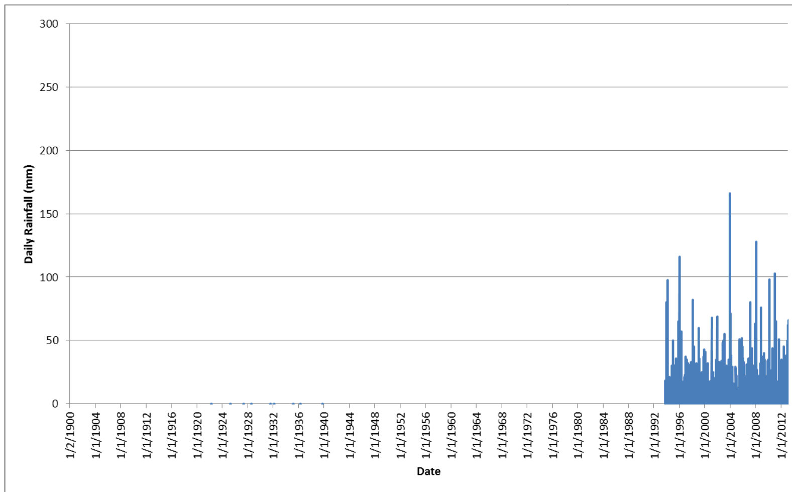
FIGURE B-21 DAILY RAINFALL: LOUDOUN BRIDGE (41339), 1900-2012
