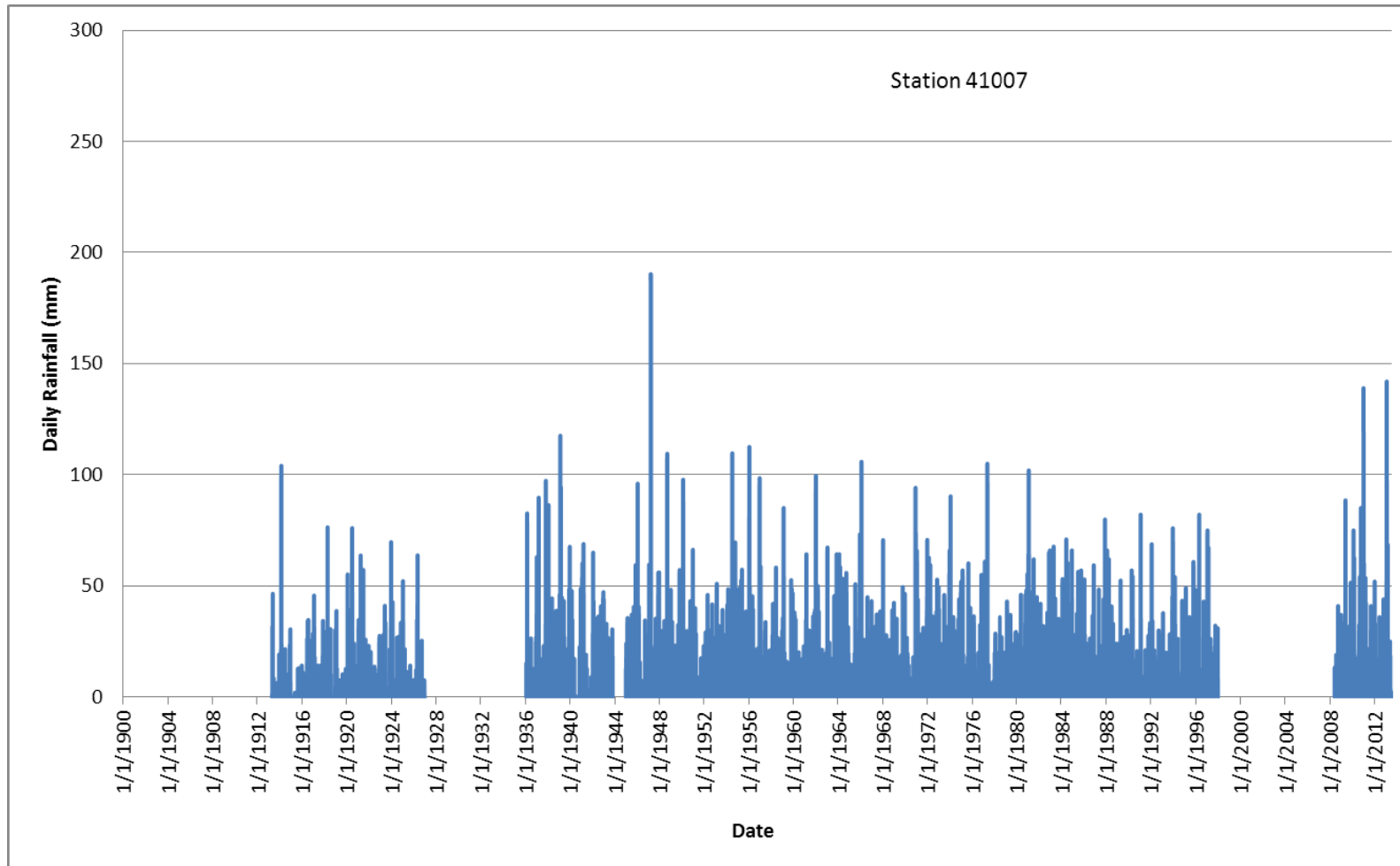
FIGURE B-5 DAILY RAINFALL: BRIGALOW POST OFFICE (41007), 1900-2012
