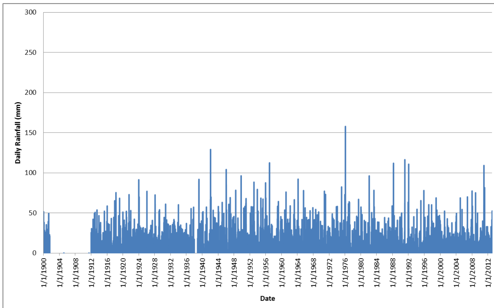
FIGURE B-7 DAILY RAINFALL: CANNING DOWNS (41013), 1900-2012
