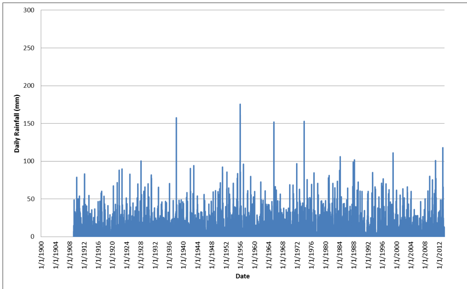
FIGURE B-11 DAILY RAINFALL: GOOMBUNGEE POST OFFICE (41037), 1900-2012
