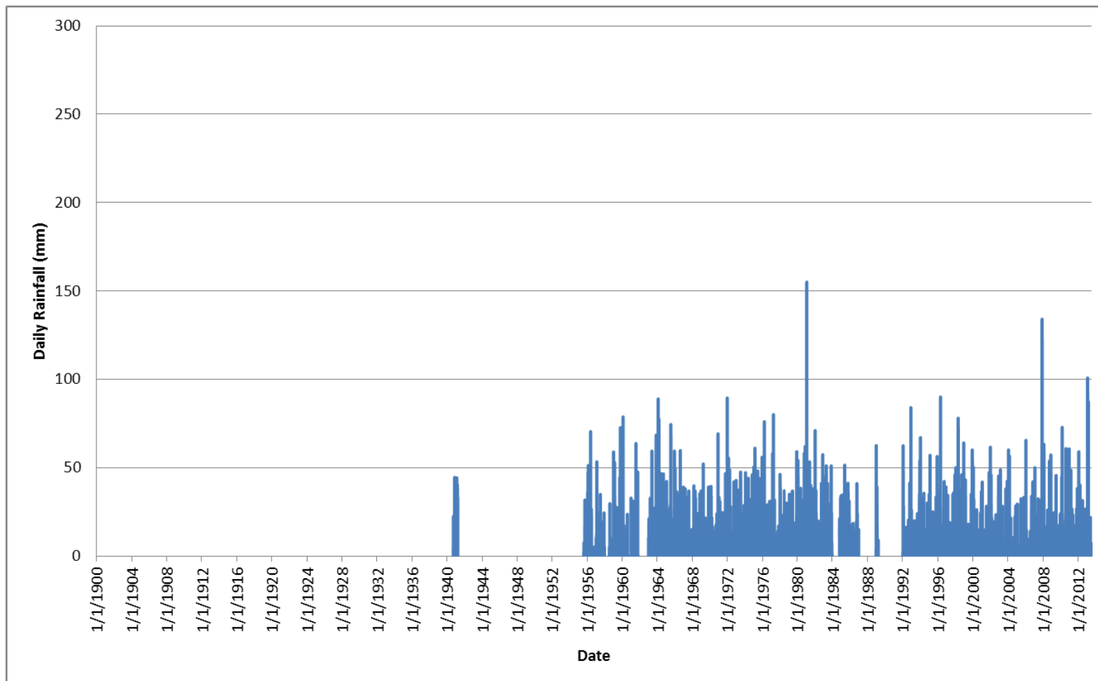
FIGURE B-18 DAILY RAINFALL: COORANGA NORTH (41131), 1900-2012
