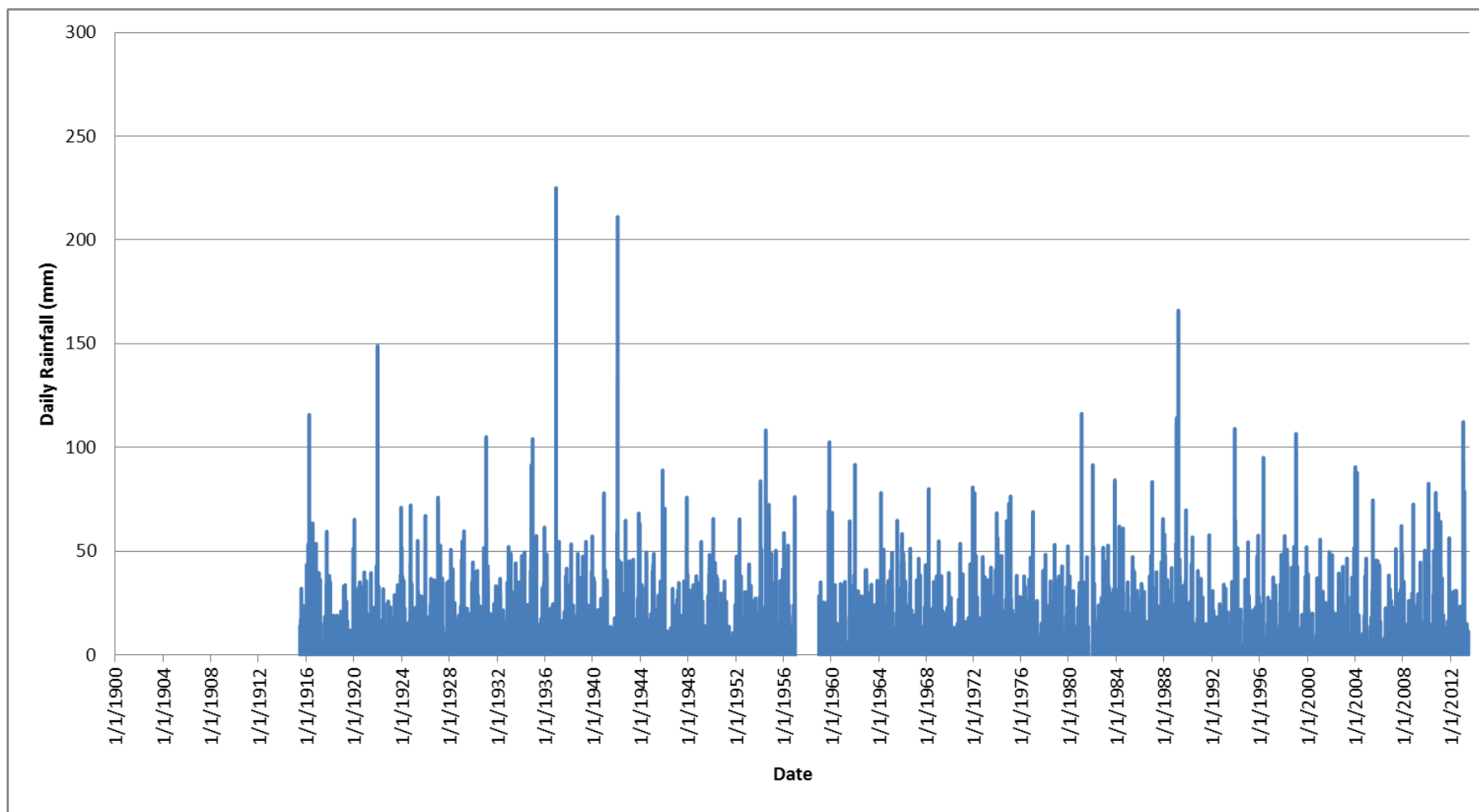
FIGURE B-12 DAILY RAINFALL: JINGI JINGI (41052), 1900-2012
