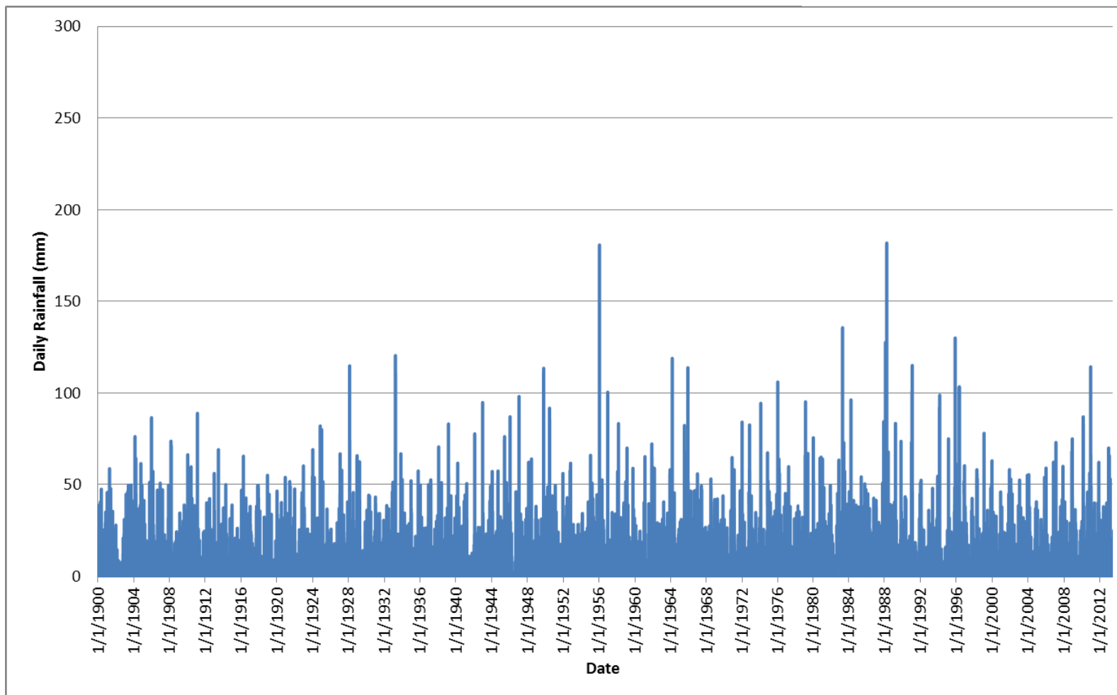
FIGURE B-16 DAILY RAINFALL: PITTSWORTH (41082), 1900-2012
