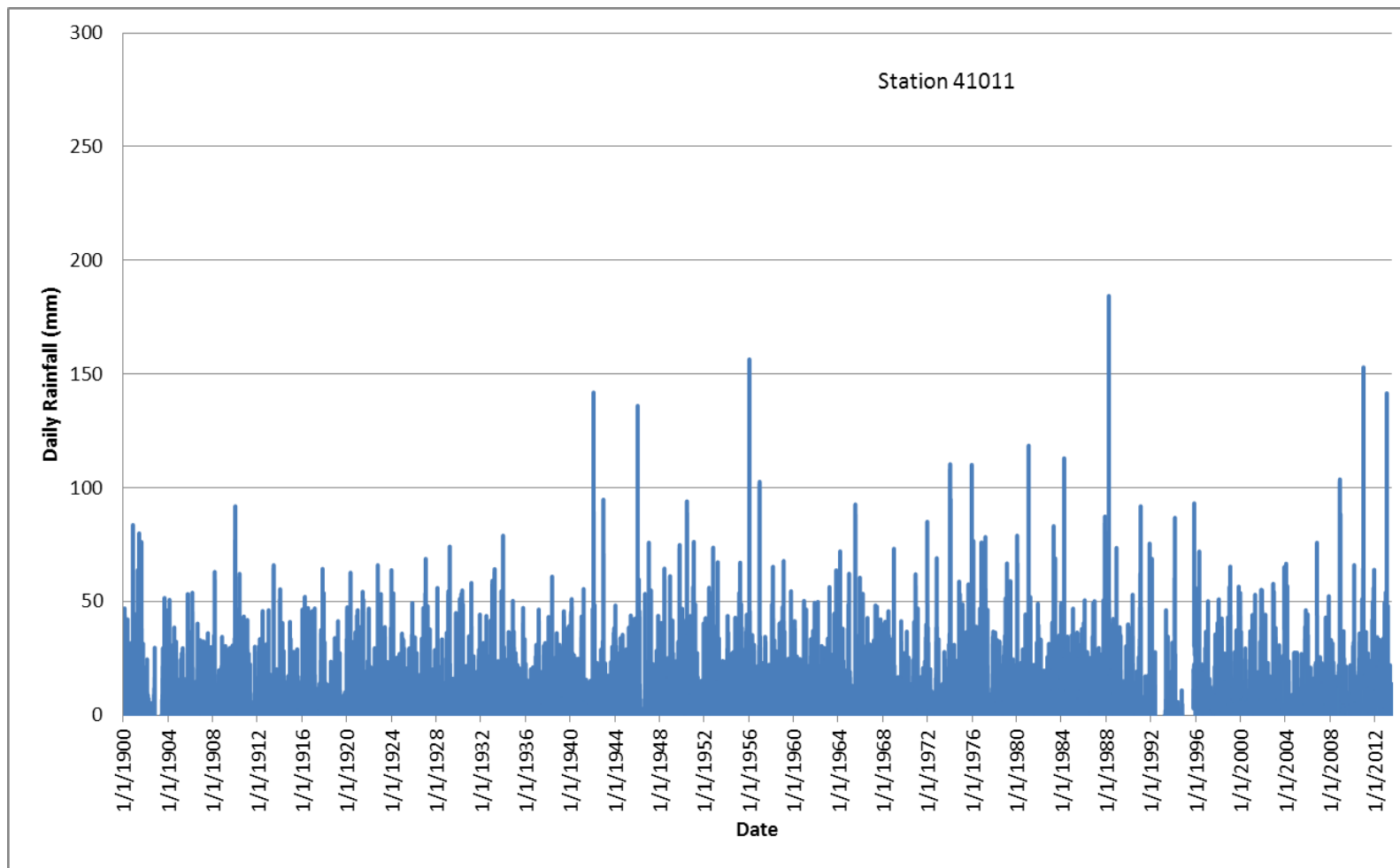
FIGURE B-6 DAILY RAINFALL: CAMBOOYA POST OFFICE (41011), 1900-2012
