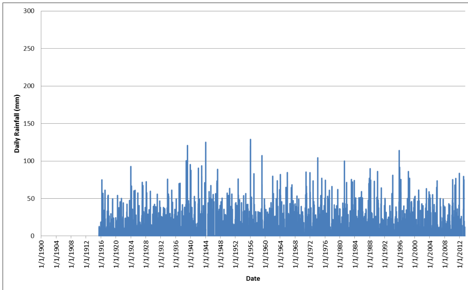
FIGURE B-14 DAILY RAINFALL: KURROWAH (41061), 1900-2012
