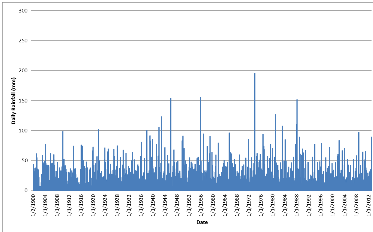
FIGURE B-13 DAILY RAINFALL: JONDARYAN POST OFFICE (41053), 1900-2012
