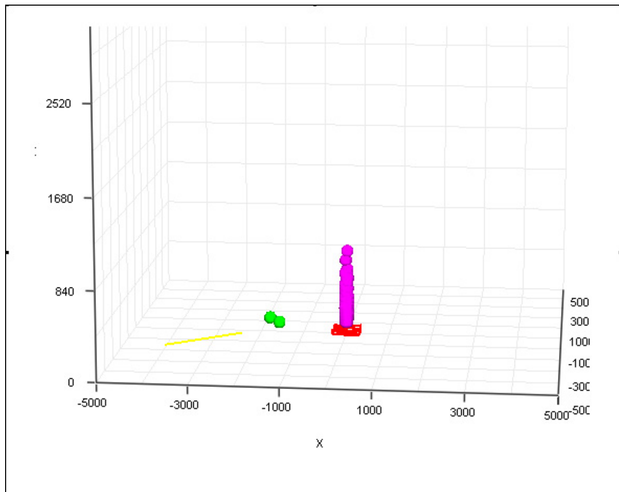
Figure 5.2 3D Representation of the Gas Processing Facility Emission Plumes (Graphis 2007)
