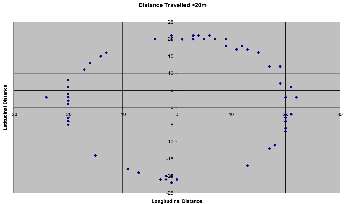
Figure 5.4 Distances Travelled >20 m at Critical Velocity
