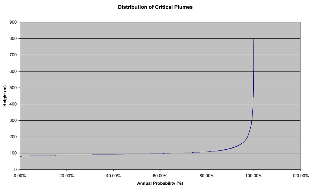
Figure 5.3 Cumulative Distributions of Critical Plume Heights
