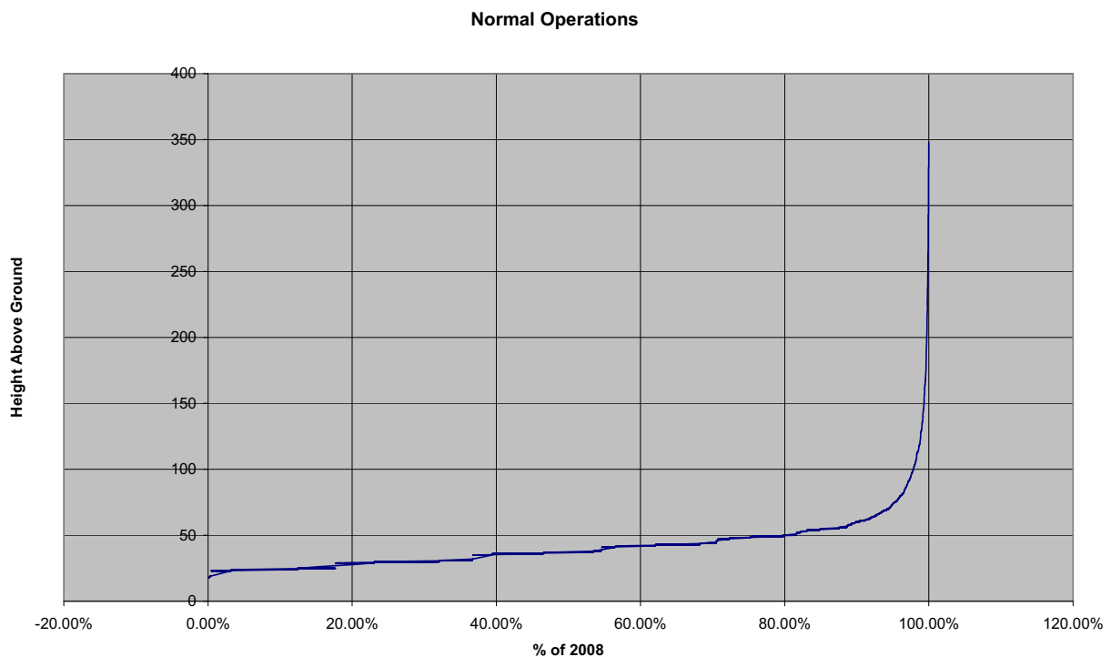
Figure 5.5 Cumulative Distributions of Critical Plume Heights
